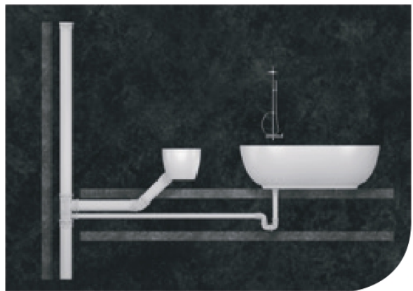
Fig. 16: Correct entry into a downpipe.
