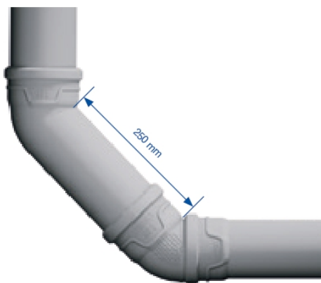
Fig. 12: Wavin AS+ long bend.
