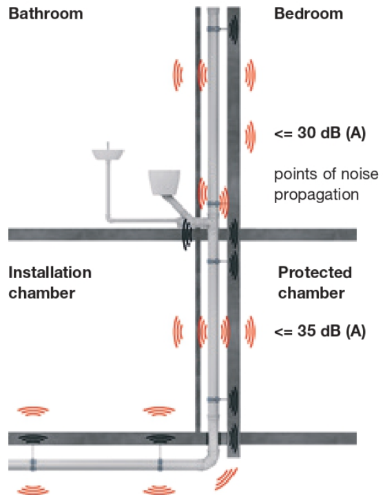
Fig. 5: Example of noise propagation during drainage.
