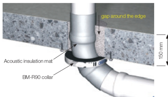
Fig. 49: Angled ceiling installation \leq 45^\circ with / without sleeve socket.
