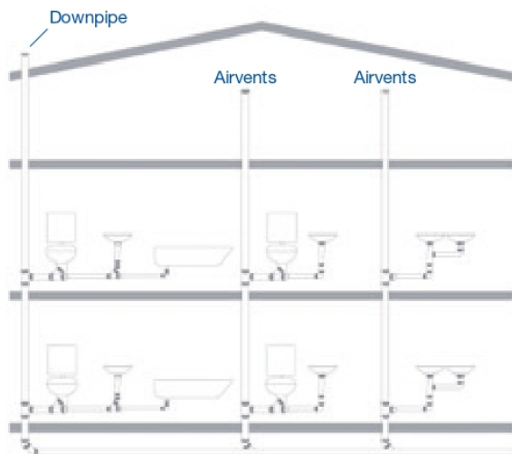
Fig. 25: Use of ventilation valves in single/two-family residential properties.
