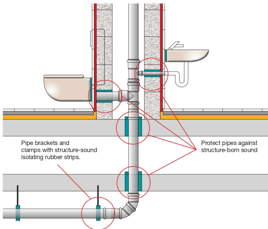
Fig. 9: Sound insulation of waste water systems.
