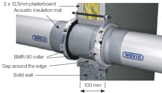
Fig. 50: Straight installation with sleeve / socket.
