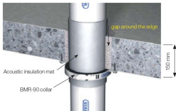
Fig. 48: Straight installation with / without sleeve / socket.
