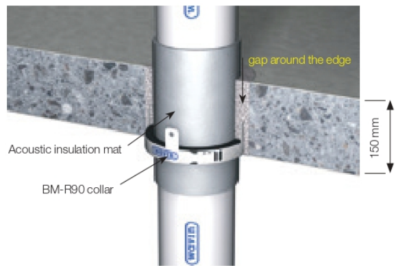
Fig. 44: Straight installation with / without sleeve / socket.
