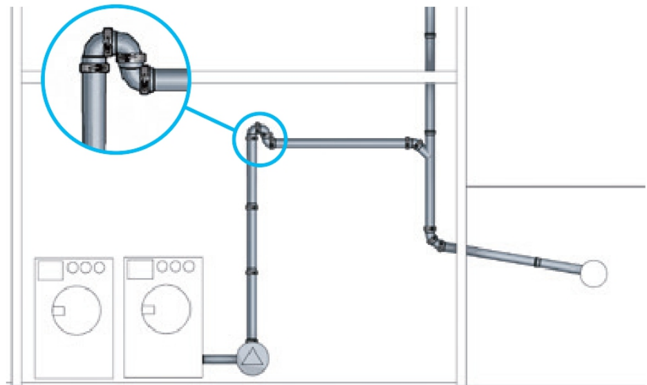
Fig. 31: Thrust resistant connector.
