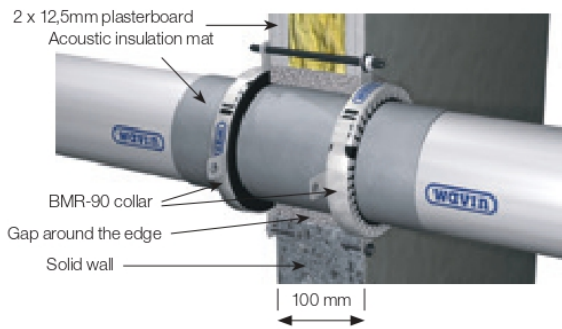
Fig. 51: Straight installation without sleeve / socket.
