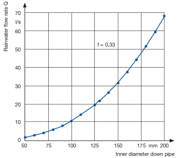
Fig.: 26: Drainage performance of rainwater downpipes.
